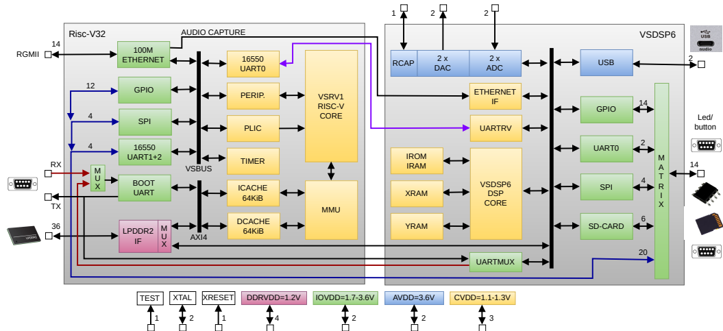
Figure 1: VSRVES01 block diagram
