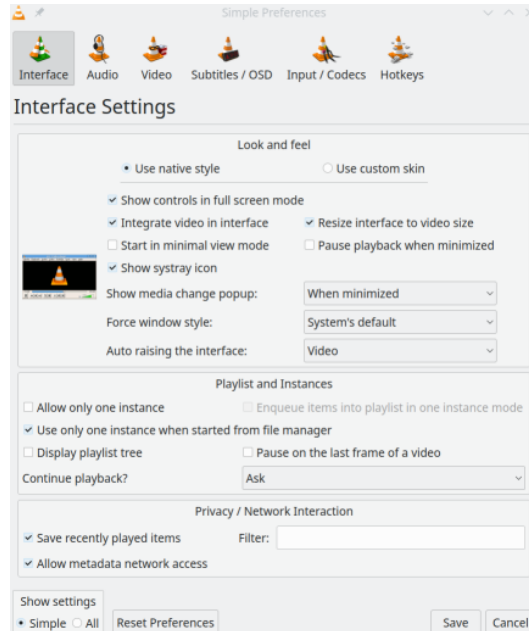
Figure 4: VLC Interface Settings, Show settings = Simple
